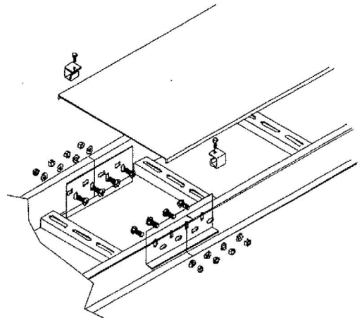
SPLICE PLATE - OUTWARD C TYPE
