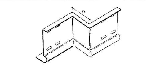
FLAT-TYPE HOLD DOWN CLAMP
